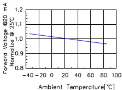
Fig 3. Forward Voltage vs. Temperature
